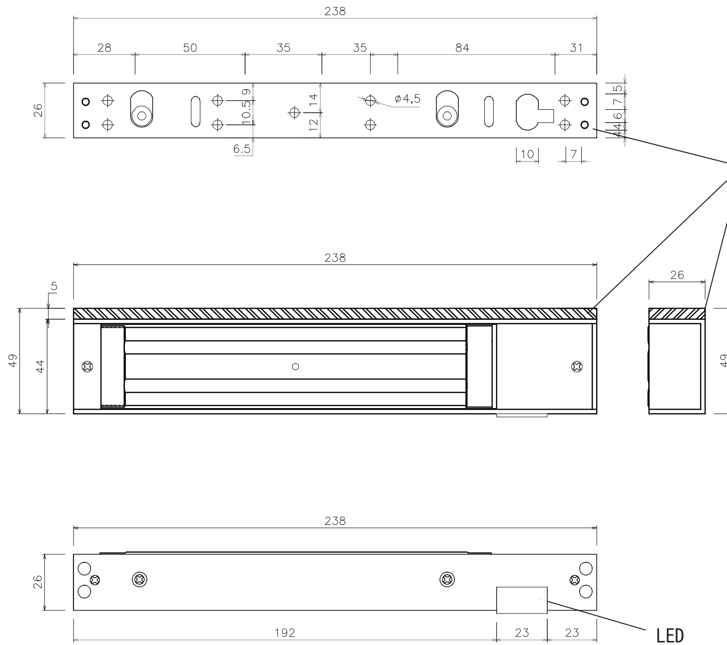
Mounting plate
